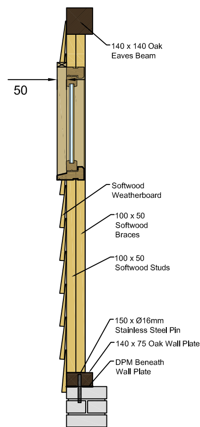
Detail H Typical Section Through Stud Wall Construction With Barn Window
