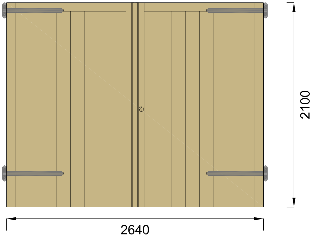
1 No. Garage Doors
