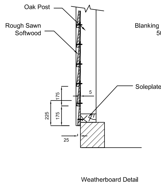
Weatherboard Detail
