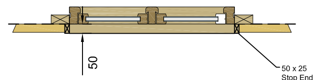
Section Through Window
